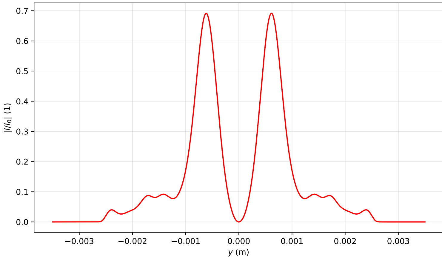
Intensity profile I(x = 0, y, z = 3.025)/I_0 , P_{in}=5.0P_{cr} , artificial time
